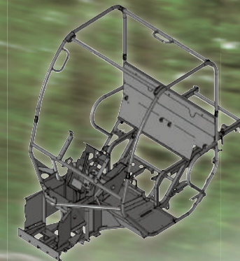
Robust Structural Frame with Standard Roll Over Protective Structure (ROPS)
